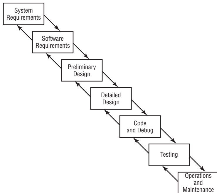
FIGURE 20.2 The waterfall lifecycle model
