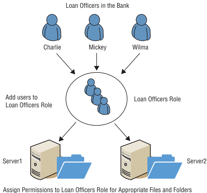
FIGURE 14.2 Role Based Access Control
