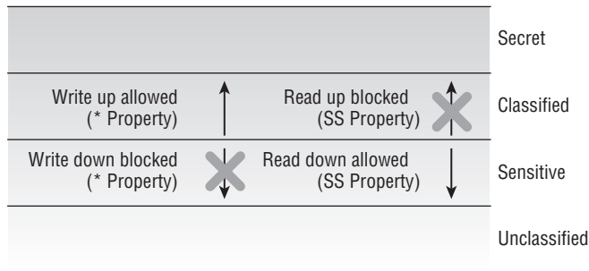
FIGURE 8.3 The Bell-LaPadula model
