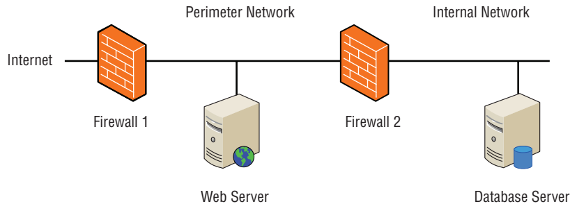
FIGURE 16.3 Web server and database server
