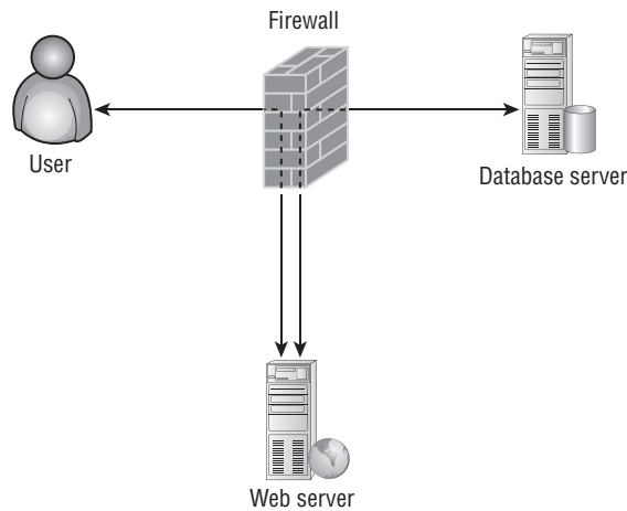
FIGURE 21.2 Typical database-driven website architecture
