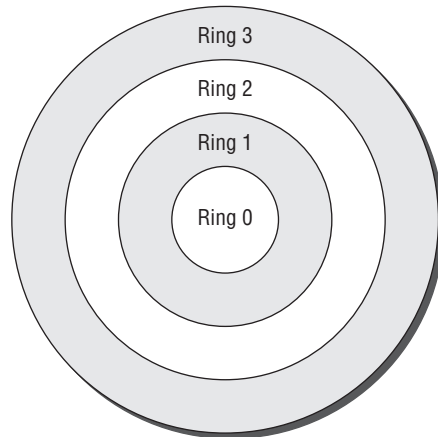
FIGURE 9.1 In the commonly used four-ring model, protection rings segregate the operating system into kernel, components, and drivers in rings 0 through 2 and applications and programs run at ring 3.
